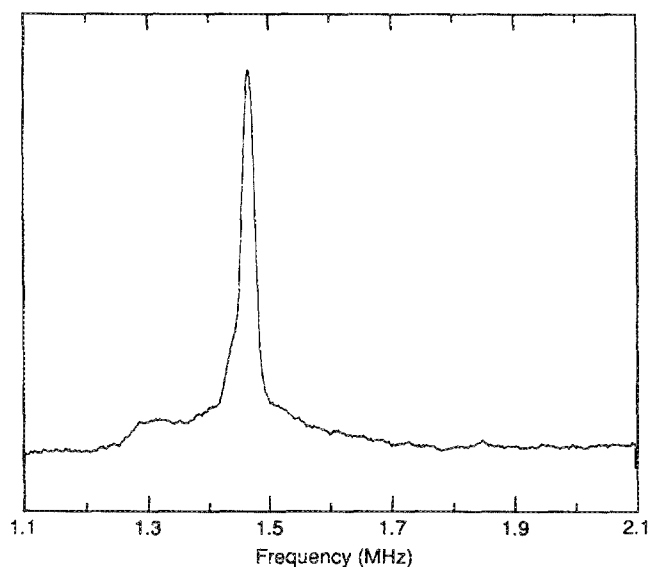
FIG. 4. NQR spectrum of boron-11 in 0.20 \text{ cm}^3 of boron nitride powder, with a dc field of 0.36 \text{ mT} . This spectrum is the difference between 10 forward and 10 reverse sweeps, each of 100 \text{ s} duration, using a linearly polarized rf field. The broad resonance near 1.3 \text{ MHz} , observed in the powder sample but not in a hot-pressed rod, is probably due to \text{B}_2\text{O}_3 \cdot x\text{H}_2\text{O} .
