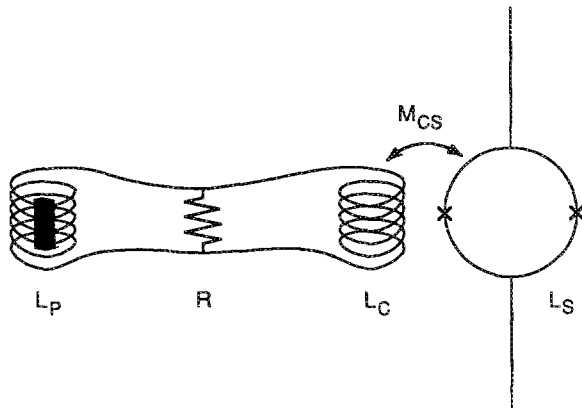
FIG. 2. Superconducting flux transformer transfers magnetic flux between the sample and the SQUID. The inductances of the pickup coil, the coupling coil, and the SQUID are L_p , L_c , and L_s respectively. R is the shunt resistance and M_{cs} is the mutual inductance between the coupling coil and the SQUID.
