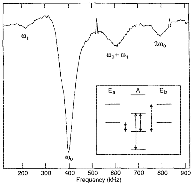
Fig. 5. Proton NMR spectrum from a single 400 s sweep of propionic acid at 4.2 K, in a field of 9.3 mT. A sample volume of 0.20 cm 3 was used. The transition between states of the same symmetry, at \omega_0 = 395 kHz, is flanked by transitions between states of different symmetry, at \omega_t and \omega_0 + \omega_t . The tunnel splitting \omega_t , is measured as 210 kHz. Also visible is the \Delta m = 2 transition at 2\omega_0 , near 800 kHz. The inset shows the energy levels for the methyl group.
