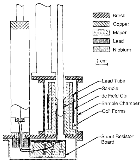
FIG. 1. Cross section of the low-temperature part of the SQUID spectrometer.
