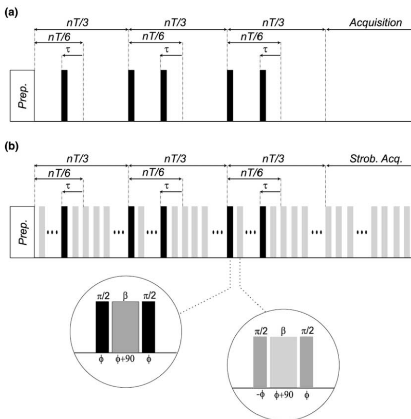
Fig. 1. (a) Basic MAT pulse timing. After initial excitation, five \pi pulses are consecutively applied during a fixed time period equal to an integer number of rotations nT (multiples of three are not allowed) [11]. In its simplest version, the second and the fourth pulses are held at nT/3 and 2nT/3 , respectively while the first, third and fifth pulses sweep along the intermediate time intervals. For a given separation of the pulses, direct acquisition is made immediately after nT . (b) In the presence of matched rf and field gradients, inhomogeneities can be periodically refocused by a train of composite z -rotation pulses. Stroboscopic acquisition at the induced (nutational) echo maxima provides an FID free of field inhomogeneities while keeping the chemical information [5]. \pi pulses can be easily merged into the train by simply reversing the phase in one of the \pi/2 -pulses. If nT/6 equals exactly an integer number of train periods, an MAT-like experiment can be performed by selectively reversing the overall phase on five of the (composite) \pi/2 pulses as shown. The latter condition, easily achievable in the rotating field case, can be satisfied in general by adjusting the free evolution interval and the duration \beta .
