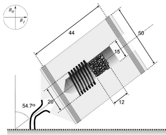
Fig. 2. Experimental setup used to simulated the ‘ ex situ ’ magic-angle field spinning. A sedimentary rock (Berea sandstone) shaped as a cylinder ( \phi = 12 mm, h = 12 mm) spins at the magic angle ( 54.7^\circ ) at about 200 Hz. The rock sits close to the edge but outside the rf coil used for excitation and detection and inside a 15-mm zirconia rotor. A pair of Maxwell coils induces an adjustable field gradient along the B_1 axis, not along the rotation axis as it first seems [13]. The homemade probe head rests inside a superwide bore 4.2 T magnet operated by a Varian/Chemagnetics Infinity spectrometer. All distances are given in mm.
