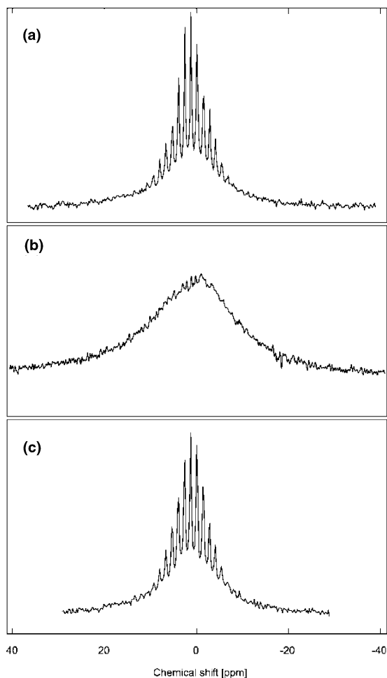
Fig. 3. One-dimensional NMR proton spectra of a porous rock saturated with water and spinning at 221 Hz. (a) With no gradient applied and inside a fairly homogeneous field, the proton spectrum displays a broadening, of the order of 15 ppm (2.7 kHz), induced by paramagnetic impurities on the walls of the pores. Because this anisotropic interaction is inhomogeneous, the profile breaks into narrow sidebands even at low spinning rates as recorded after a single \pi/2 pulse excitation (8 scans). (b) Same experiment but in the presence of a gradient of 8 kHz/cm, resulting in a broadening of the line profile (32 scans). (c) Even in this gradient, rotational echoes (and, with them, the original shape of the spectrum) are almost completely recovered by means of a train of refocusing composite z -rotation pulses. The series (2\gamma)_{97.2}(4\gamma)_{291.5}(2\gamma)_{97.2}(\gamma)_0 was used as a composite \pi/2 pulse [14]. The nominal 90^\circ length \gamma was 5 \mu s and the free evolution period was 47 \mu s; \beta was 17 \mu s and the number of rotor periods n was 2.
