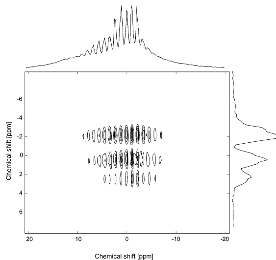
Fig. 4. Two-dimensional proton spectrum of pure ethanol contained in the rock after running a modified MAT experiment shown in Fig. 1. The gradient along the sample was 8 kHz/cm and the spinning speed was 214 Hz. The direct dimension in which the slow spinning sideband spectrum appears is plotted horizontally: due to strong overlapping; no clear indication of ethanol can be discerned from the spectrum. The indirect dimension, displaying the isotropic chemical shifts, is plotted vertically and, despite some residual broadening, the expected pattern can be clearly recognized. As a reference, the resolution of \sim 1 ppm can be compared with that of Fig. 3(b), \sim 10 ppm.
