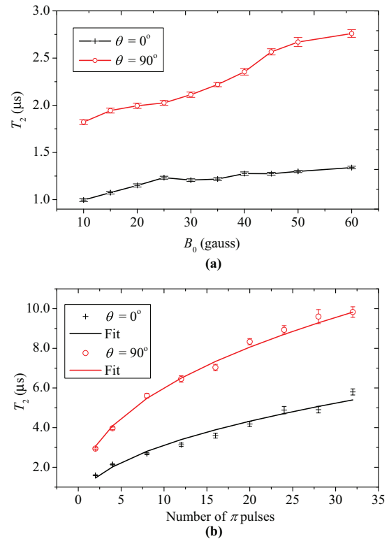
FIG. 4. (Color online) (a) Spin-coherence time as a function of the amplitude of a magnetic field applied parallel to the NV axis ( \theta = 0^\circ ), or perpendicular to the NV axis ( \theta = 90^\circ ). (Solid lines serve to guide the eye.) (b) Spin-coherence time of ensemble NV centers as a function of the number of \pi pulses ( N ) in the CPMG pulse sequence at \sim 75 G applied parallel or perpendicular to the NV quantization axis. Solid lines are fits to T_2 \sim N^r with r = 0.47 \pm 0.04 for \theta = 0^\circ and 0.42 \pm 0.01 for \theta = 90^\circ .
