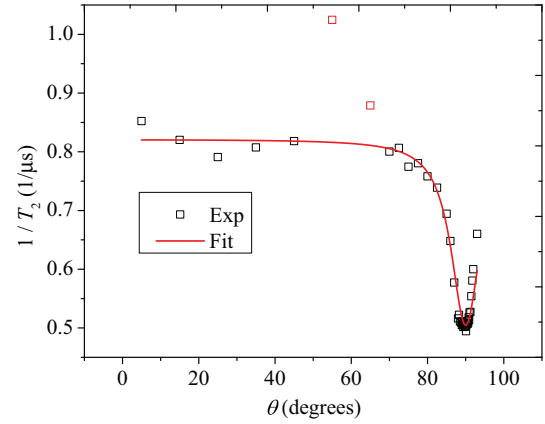
FIG. 3. (Color online) Coherence decay rate ( 1/T_2 ) as a function of magnetic field orientation ( \theta ) with respect to the NV axis at \sim 25 G. The solid line is a fit of experimental data ( 1/T_2 ) to Eq. (10) using \tau_0 as a free parameter, together with an offset that accounts for the residual noise contributions. The value \gamma b_z/2\pi \sim 0.69 \pm 0.01 MHz was estimated from the free induction decay, while E/2\pi \sim 4.85 MHz was estimated from the ODMR spectrum at ambient field. The outliers at 55^\circ and 65^\circ , which might be affected by NV centers in other orientations, were not included in the fitting.
