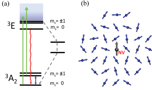
FIG. 1. (Color online) (a) Energy level structure of the NV center showing spin triplet ground ( {}^3A_2 ) and excited ( {}^3E ) states with single states (green arrows for optical excitation at 532 nm, red arrow for fluorescence decay, gray arrows for nonradiative decay via singlet states, and blue arrow for microwave excitation). (b) Schematic of an NV center spin, coupled to bath spins dominated by substitutional nitrogen (P1) spins (blue balls with arrow for P1 spins).
