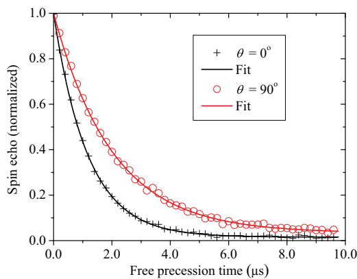
FIG. 2. (Color online) Coherence decay of ensemble NV electron spins with an external magnetic field of \sim 25 G applied parallel or perpendicular to the NV quantization axis (solid lines are fits to a single exponential decay). The measured coherence time was 1.17 \pm 0.01 \mu\text{s} for \theta = 0^\circ (crosses) and 2.01 \pm 0.01 \mu\text{s} for \theta = 90^\circ (circles).
